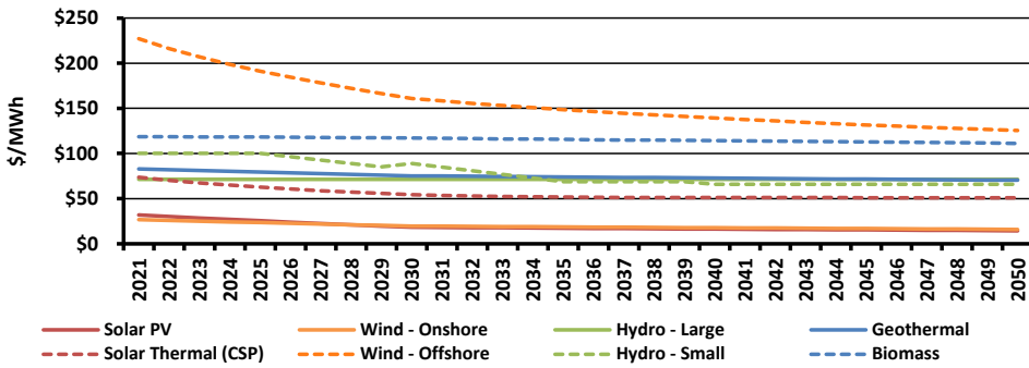
Figure 6 – Forecast Levelized Cost of Renewable Electricity Generation Technology
